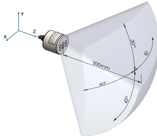
Fig. 12. The RBR tridente with the recommended unobstructed volume. The machined mark above the middle window serves as a reference for the detector windows. The mark is also used for orientation, indicating the top direction.
