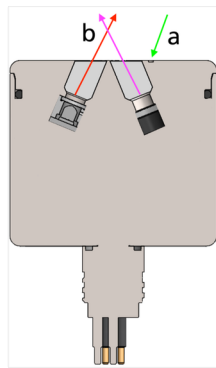
Fig. 9. Cross section of the RBR tridente . (a) Machined mark. (b) Angled detector-LED pair, with red and pink arrows, respectively.
