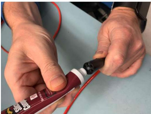
Fig. 12. Applying silicone compound to the female connectors.
