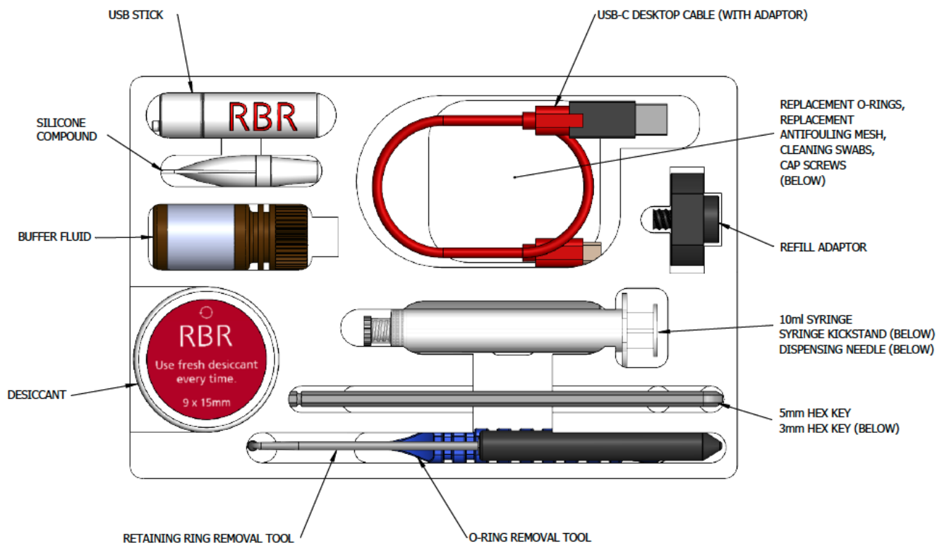
Fig. 6. RBRquartz³ support kit diagram
