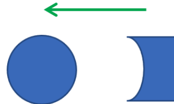
Fig. 13. Orientation of the O-rings. Left: main O-ring, right: backup O-ring
