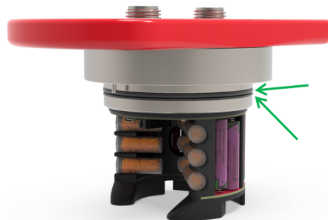
Fig. 12. Location of the O-rings. Top: main O-ring, bottom: backup O-ring
