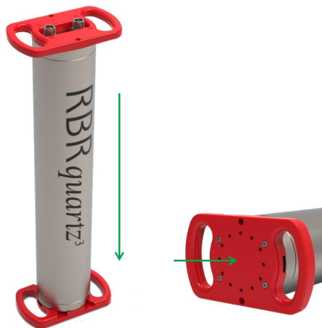
Fig. 7. Left: recommended orientation, sensor end-cap down; right: datum location
