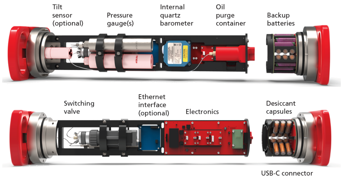
Fig. 1. RBRquartz 3 BPR | zero
