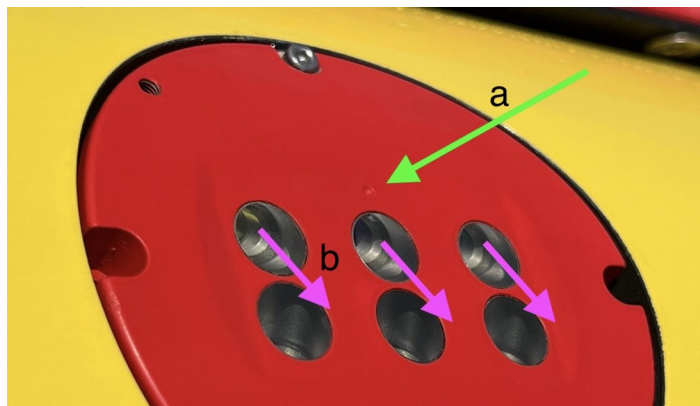
Fig. 8. An RBR tridente mounted horizontally. (a) Machined mark. (b) The downward direction of the detectors.
