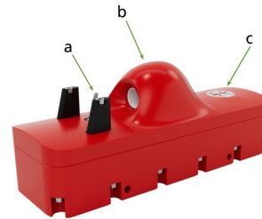
Fig. 2. Side view of an RBR legato 4 C.T.D. (a) Temperature sensor. (b) Conductivity sensor. (c) Pressure sensor.
