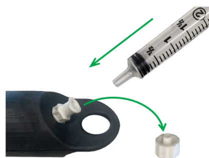
Fig. 9. Gently push down the piston to inject until full
