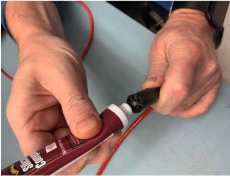
Fig. 10. Applying silicone compound to the female connectors.
