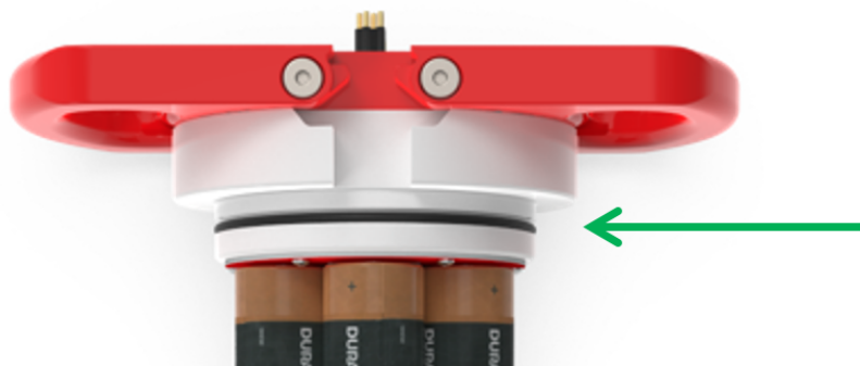
Fig. 8. Location of the O-ring
