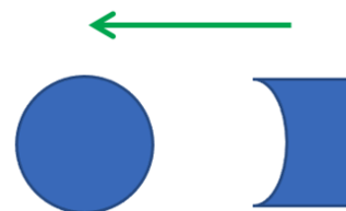
Fig. 9. Orientation of the O-rings (Main O-ring, Backup O-ring)
