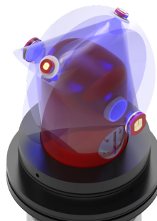
Fig. 2. Four UV LEDs illuminating the CT cell
