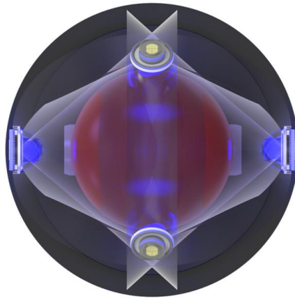
Fig. 3. Four UV LEDs illuminating the CT cell
