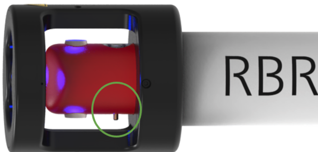
Fig. 8. CTD | uv cell, with thermistor circled
