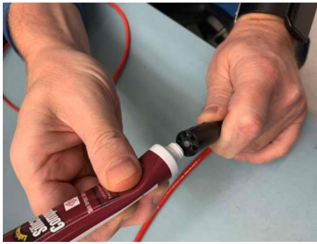
Fig. 23. Applying silicone compound to the female connectors.
