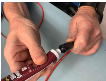
Fig. 27. Applying silicone compound to the female connectors.
