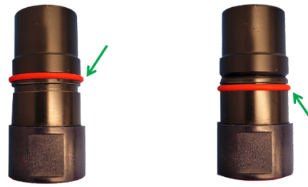
Fig. 33. Transport position (left), measurement position (right)
