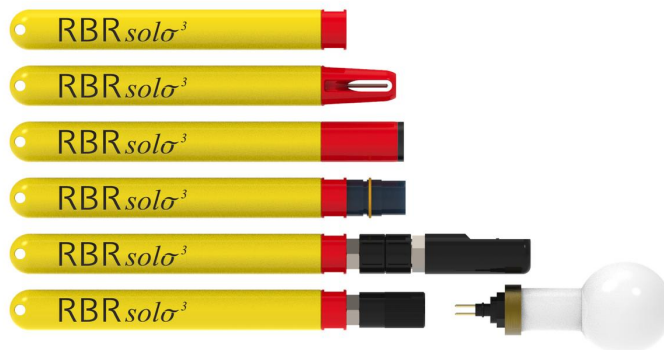
Fig. 2. The RBRsolo 3 shallow instruments
