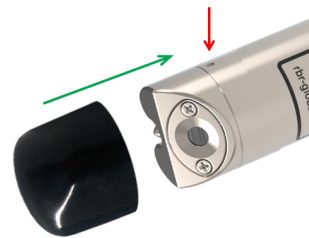
Fig. 29. The RBRcoda ODO with storage cap: note the red arrow showing the location of the locking pin
