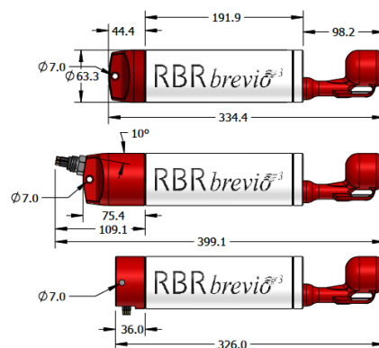
Fig. 8. RBRbrevio 3 dimensions with three different battery end-caps
