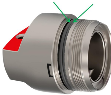
Fig. 25. Location of the O-rings, | deep: main O-ring (left), backup O-ring (right)
