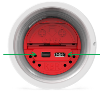
Fig. 15. Left: Mini-display port, right: USB-C port
