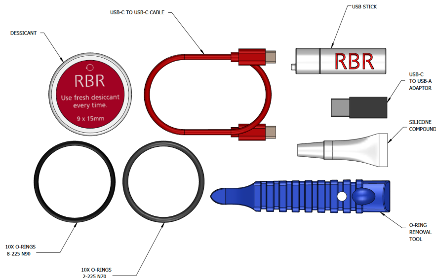
Fig. 23. RBR support kit diagram (for titanium)
