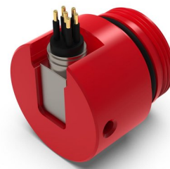
Fig. 18. Right-angle connectorised end-cap
